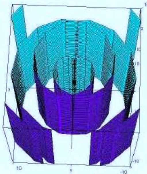
Figure 3. Involutive B-scroll of the circle.
