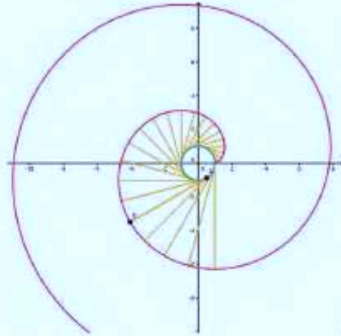
Figure 1. A circle and its involute.
