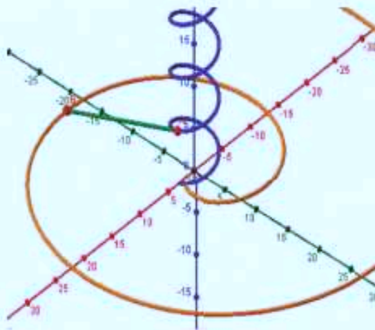
Figure 2. A helix and its involute.
