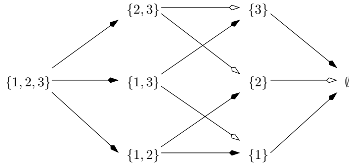
Figure 2: The 3-cube complex \mathcal{C}_*^3 . The lattice of subsets of \{1, 2, 3\} forms a 3-dimensional cube and \partial S is a signed sum of the neighbours of S of smaller cardinality. In the diagram positive terms are indicated by solid arrowheads, negative terms by empty arrowheads.
