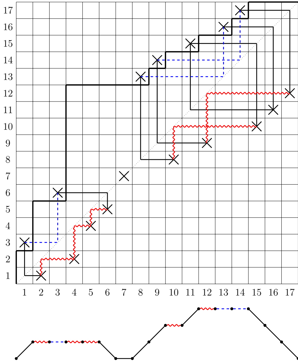
Figure 3: The associated bicolored Motzkin path.
