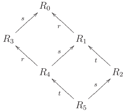
Figure 1: Hasse diagram of G
