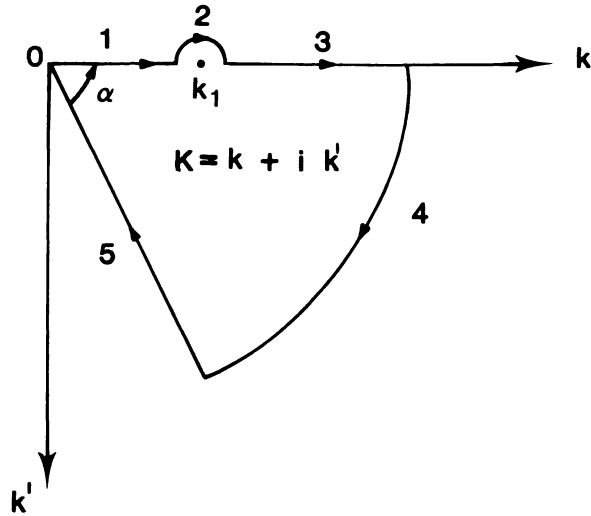
Figure 3: Closed contour for w_+ < 0
