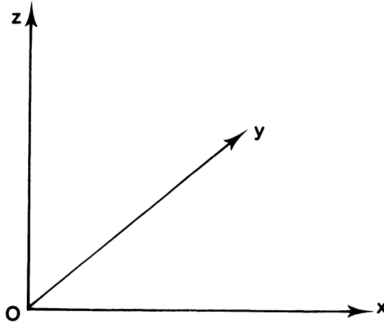
Figure 1: The Coordinate System
