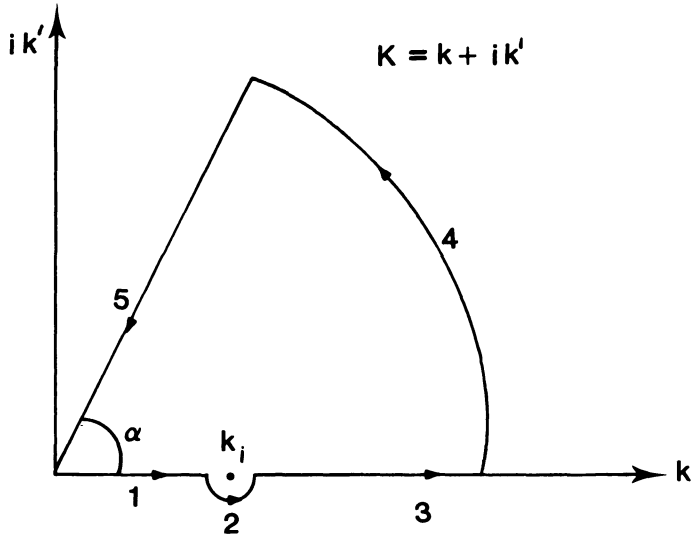
Figure 2: A closed contour for w_+ > 0
