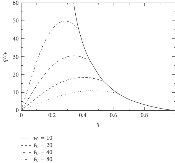
Figure 5.1. Normalized flow q/c_p versus normalized concentration \eta = c/c_p for different average desired speeds \bar{v}_0 and \tau c_p = 0.1 for the lognormal distribution with \sigma = 0.93 and \mu' = 0.83 .
