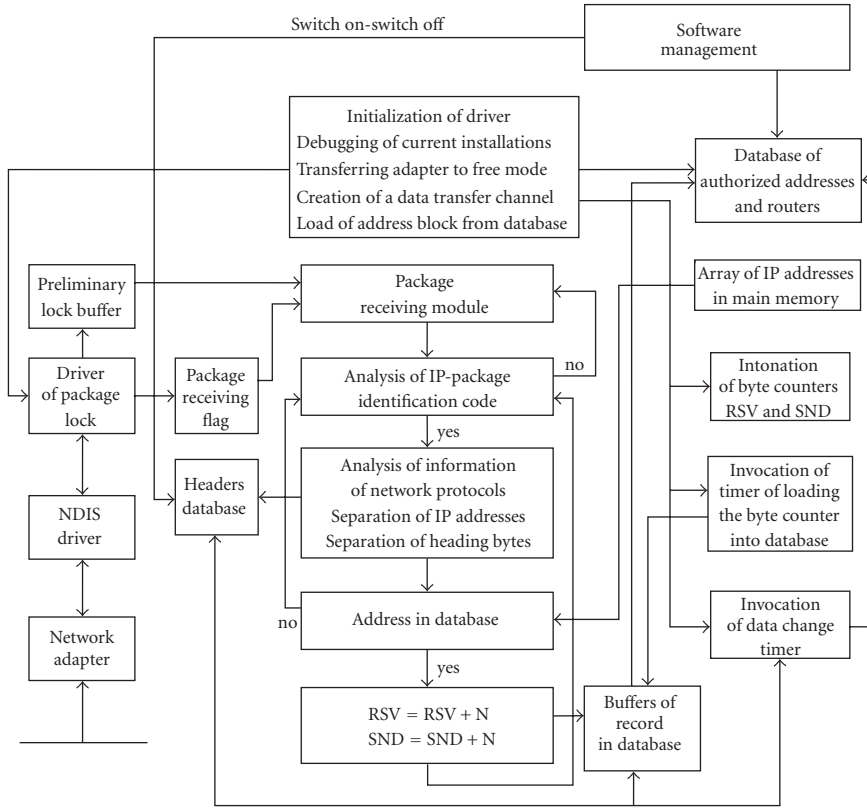
Figure 2.1. Scheme of a data acquisition system.
