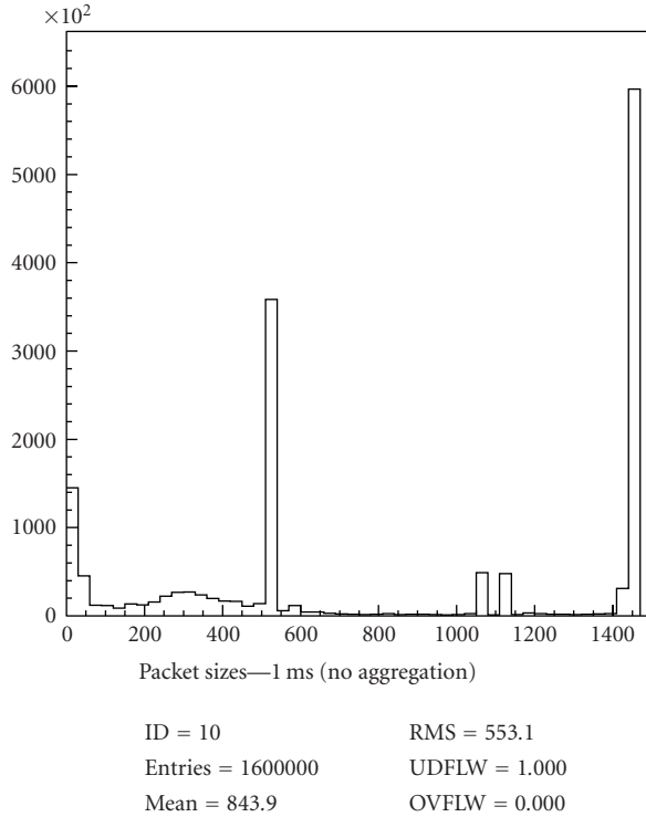
Figure 4.1. Packet size distribution for traffic measurements.
