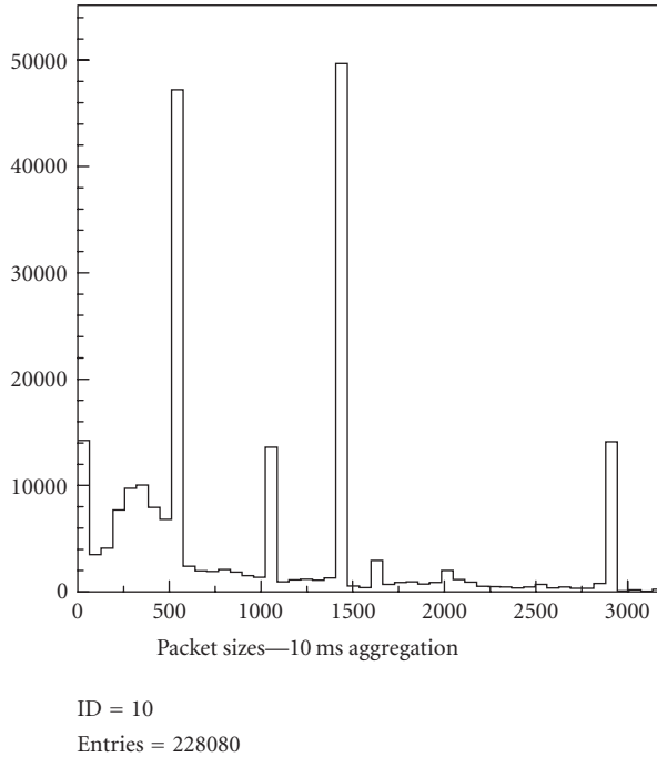
Figure 4.2. Packet size distribution for traffic measurements aggregated with bin size 10 milliseconds.
