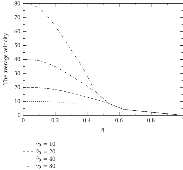
Figure 5.2. The average velocity as function of \eta = c/c_p for different average desired speeds \bar{v}_0 and \tau c_p = 0.1 for the lognormal distribution with \sigma = 0.93 and \mu' = 0.83 .
