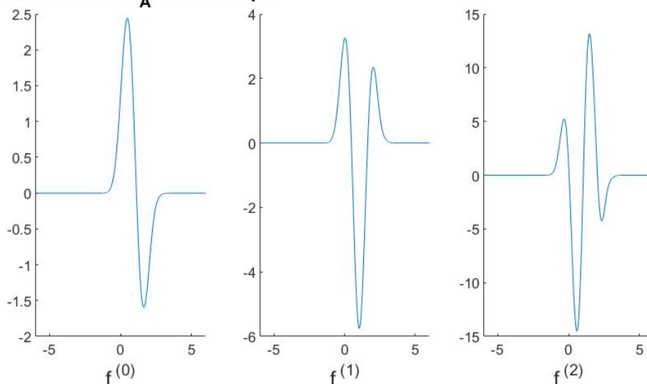
Figure 2: The function and its first and second derivatives
