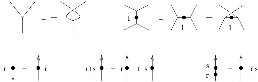
Figure 3: The AS, IHX (for arbitrary orientations of the edges), Orientation Reversal and Linearity relations. Here r \rightarrow \bar{r} is the involution of R , r, s \in R .
