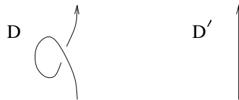
Figure 31: A type I move
