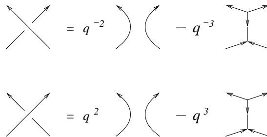
Figure 10: Decompositions of crossings
