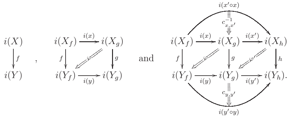
Figure 1: Objects, morphisms and the composition of the category \Lambda_i T (the diagram on the right hand side ignores the associators and the bracketing of 1-morphisms). Here, c is the compositor of the 2-functor i .
