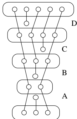
Figure 15: Example Object From \Phi^4
