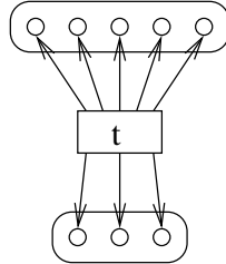
Figure 10: Object in the Groupoid of Stuff Operator T
