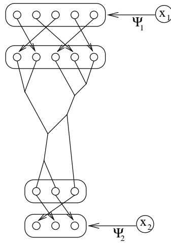
Figure 18: An Object in \langle \Psi_2, (\Phi^3 // S_3)^6 \Psi_1 \rangle
