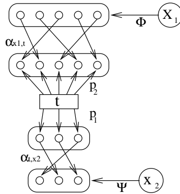
Figure 13: Object of Groupoid \langle \Psi, T\Phi \rangle
