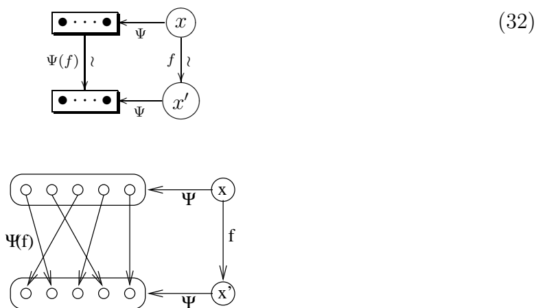
Figure 5: Morphism In the Groupoid of Stuff Type \Psi
