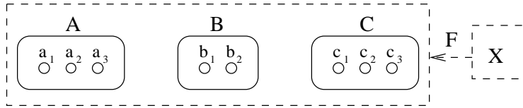
Figure 6: An Object in a Composite Stuff Type
