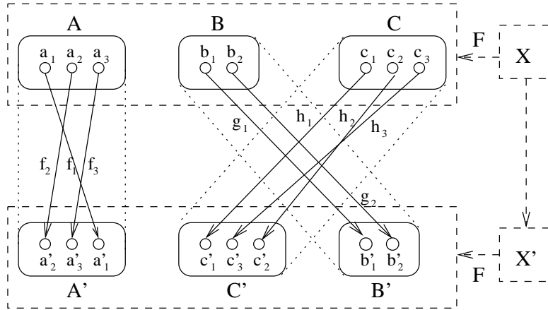
Figure 7: A Morphism in a Composite Stuff Type
