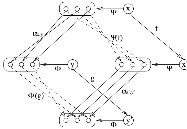
Figure 9: A Morphism in an Inner Product (Pullback) Groupoid
