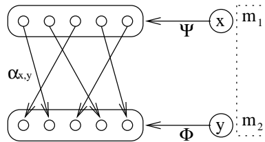
Figure 21: An Object In the Inner Product of two M -Stuff Types
