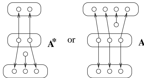
Figure 14: Example Objects in the Categorized Field Operator
