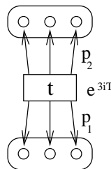
Figure 22: An Object in The U(1) -Stuff Operator E_T
