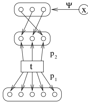
Figure 11: Object of Stuff Type T\Psi
