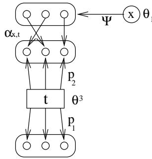
Figure 23: An Object in The U(1) -Stuff Type E_T\Psi
