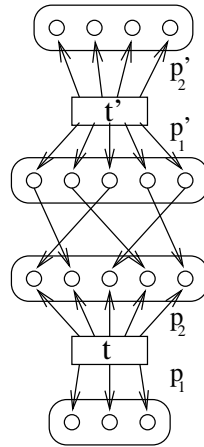
Figure 12: Object of Stuff Type TT'
