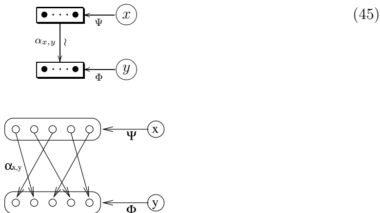
Figure 8: Object of an Inner Product (Pullback) Groupoid
