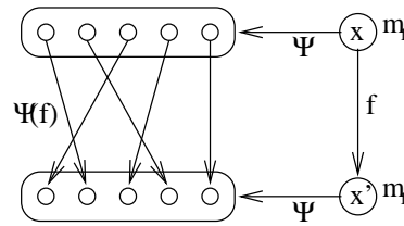
Figure 20: A Morphism in the Groupoid of an M -Stuff Type
