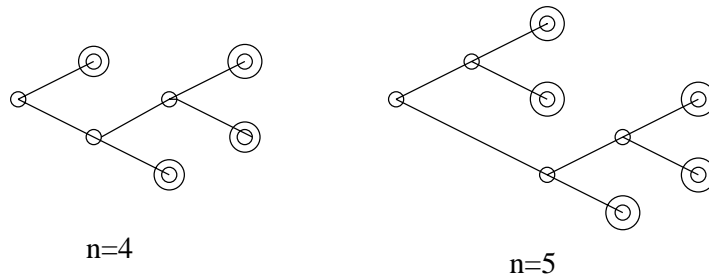
Figure 1: Some Binary Trees with n Leaves
