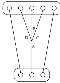
Figure 16: Example Object From \Phi^4 (Alternate Style)
