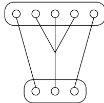
Figure 17: Example Object in \Phi^4//S_4
