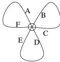
Figure 19: Example Object in \langle 1, \Phi^6 // S_6 1 \rangle
