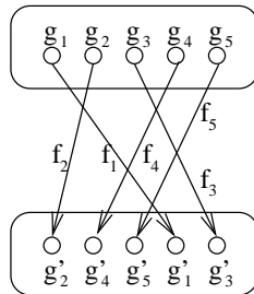
Figure 3: A Morphism of \mathcal{G} -Coloured Sets
