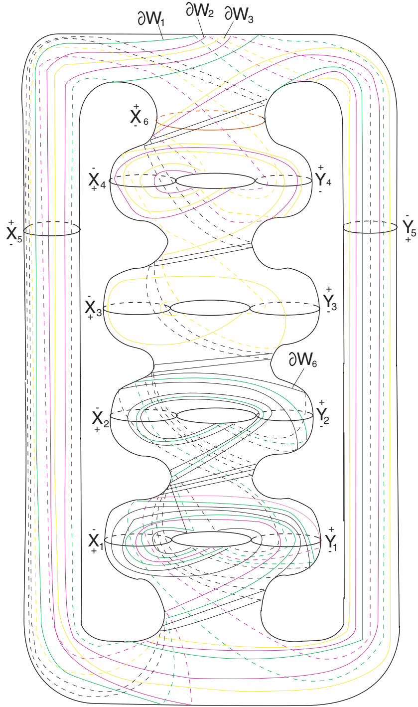
FIGURE 17. \partial W_6 = \tilde{\alpha} , \partial W_1 , \partial W_2 , \partial W_3 on the Heegaard surface \partial \tilde{H}
