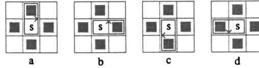
Figure 15. Four domino positions.
