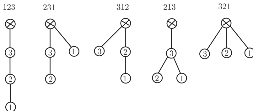
Figure 1: The five ordered trees on 3 edges and their permutations.
