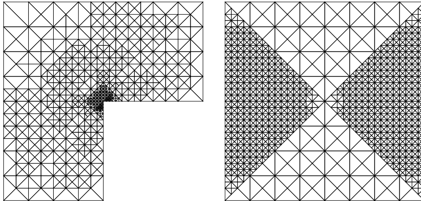
Figure 4.2a. Reentrant corner.
