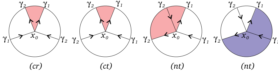
Figure 2. The angle between the paths.
