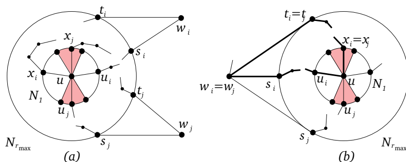
Figure 4. The construction of cycles C_1, C_2, \dots, C_N when k even.
